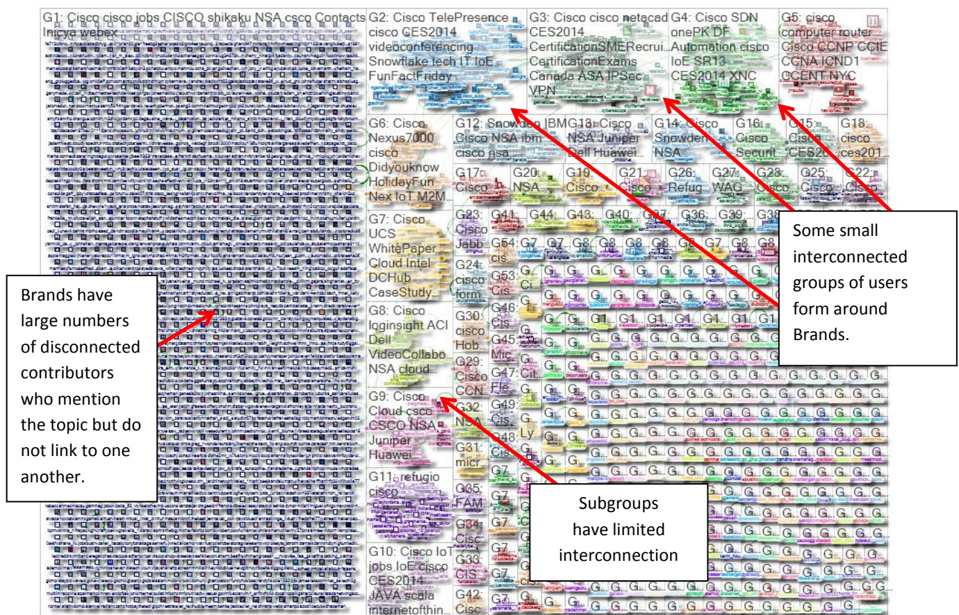
Figure 24: Network graph of 2808 Twitter users whose tweets contain the hashtag #cisco collected on January 9, 2014. There is a line or "edge" for each "replies-to" or "mentions" relationship in a tweet. There is a self-loop edge for each tweet that is not a "replies-to" or "mentions."
